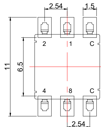
PCB LAYOUT
