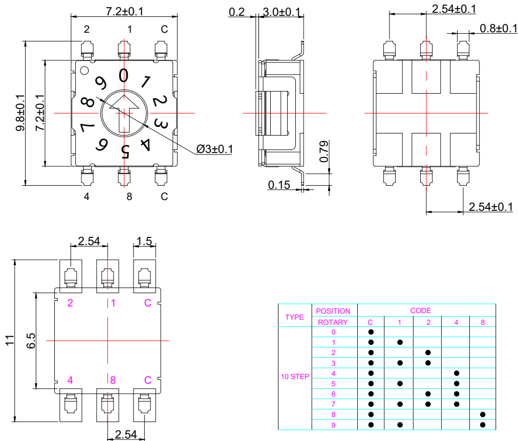
PCB LAYOUT
